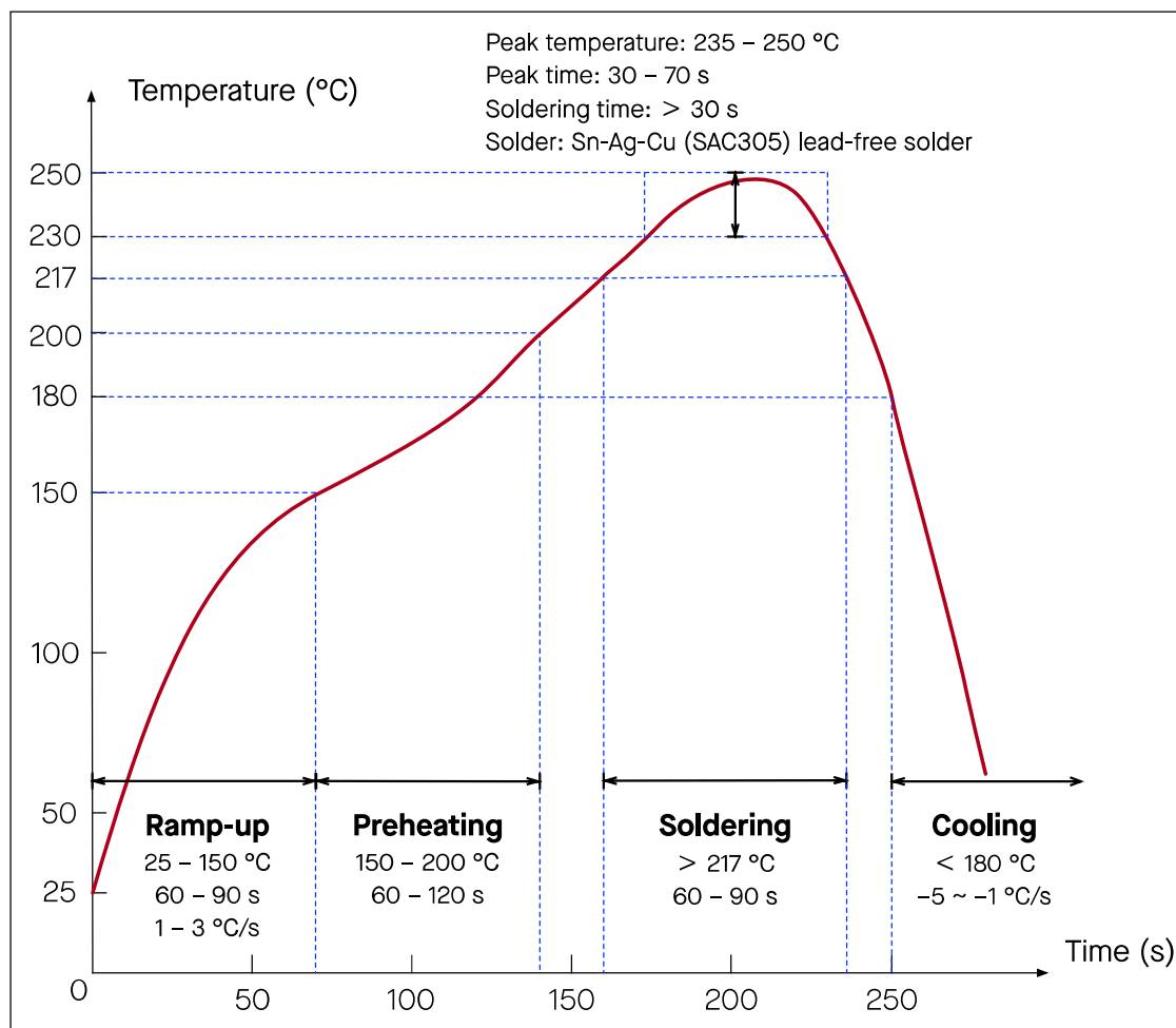
Figure 12-1. Reflow Profile
