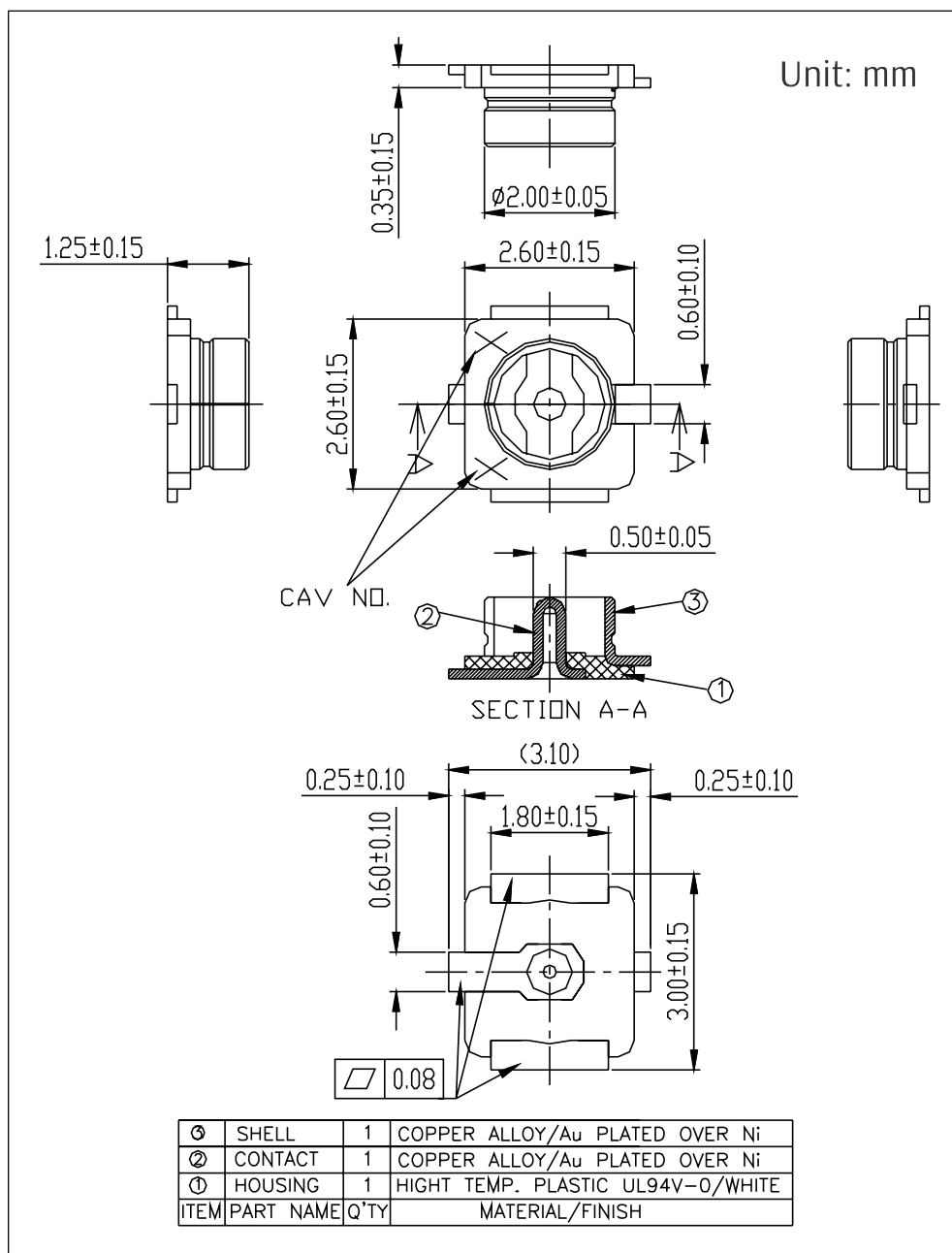
Figure 10-3. Dimensions of External Antenna Connector
