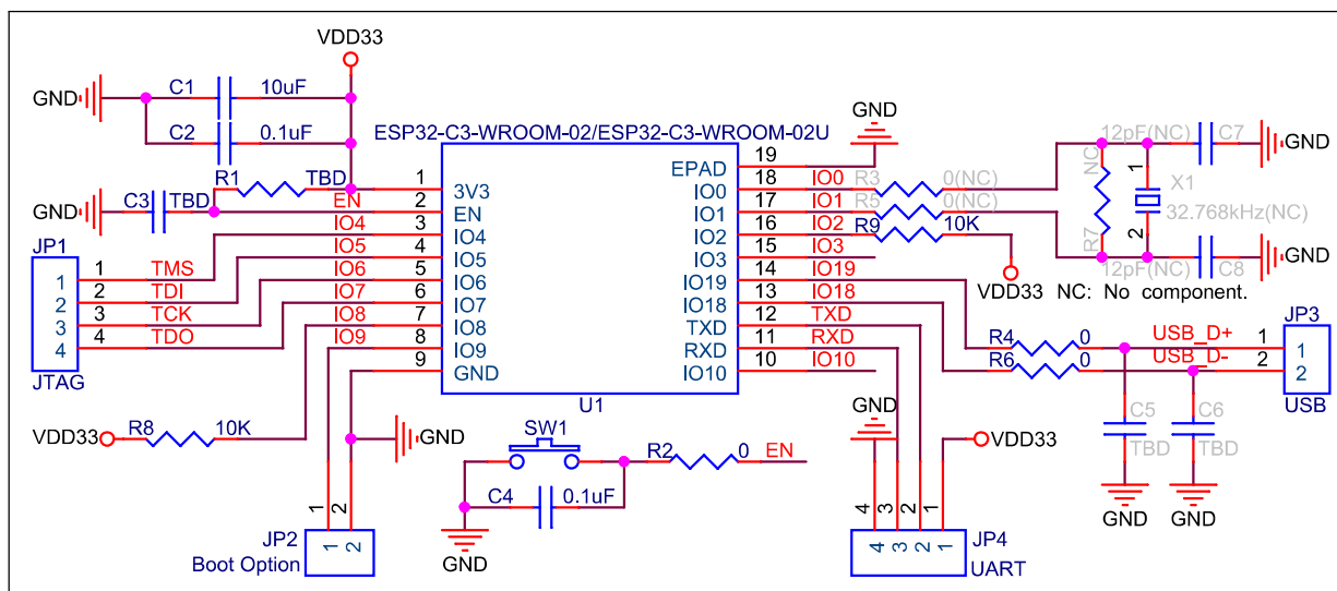
Figure 9-1. Peripheral Schematics
