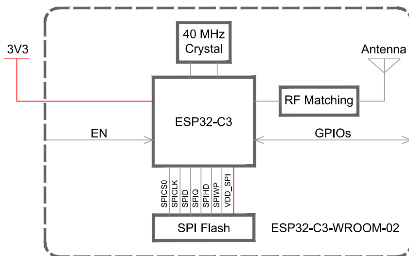
Figure 2-1. ESP32-C3-WROOM-02 Block Diagram
