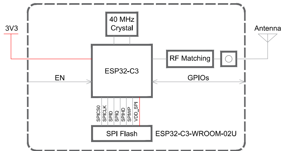
Figure 2-2. ESP32-C3-WROOM-02U Block Diagram
